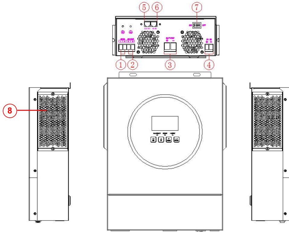
Figure 2:2250VA/4200VA model
